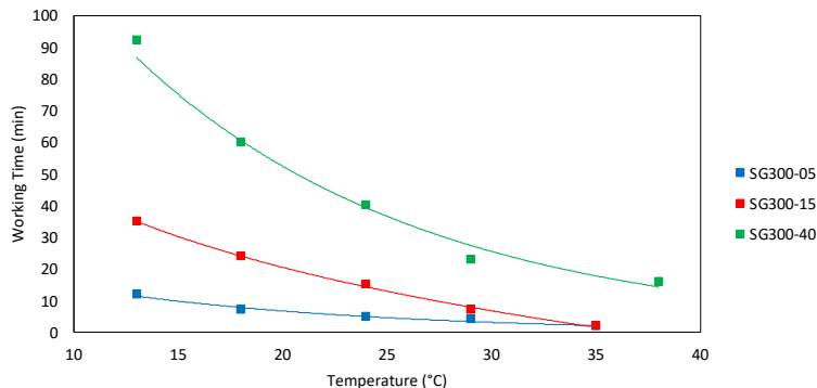
Working Time vs Adhesive Temperature
