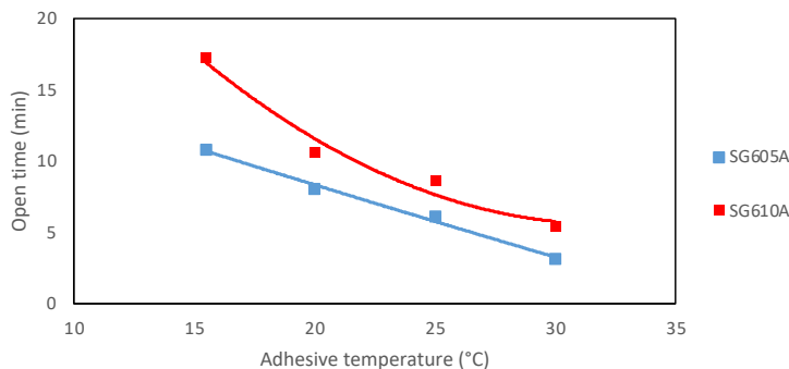
SG600 Series - Open Time vs. adhesive temperature
