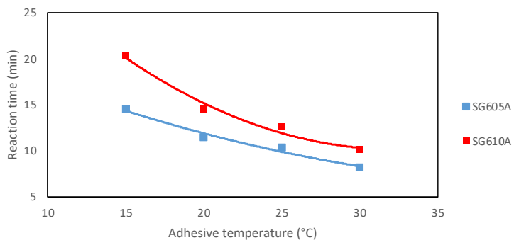
SG600 Series - Fixture time vs. adhesive temperature
