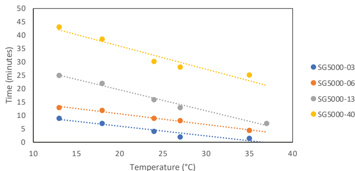
Fixture Time vs Adhesive Temperature
